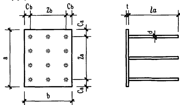
M3-1xx, M3-2xx
